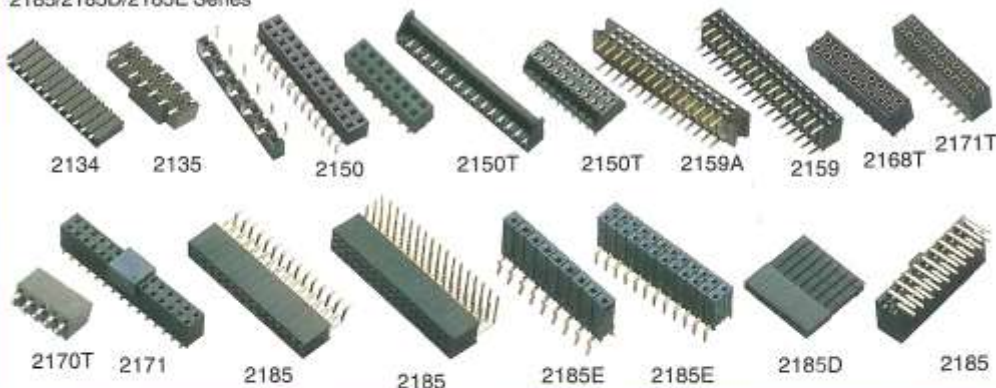
2.54mm Female Header:2134/2135/2136T/2145/2150/2150T/2159/2168/2168T/2170/2170T 2185/2185D/2185E Series
